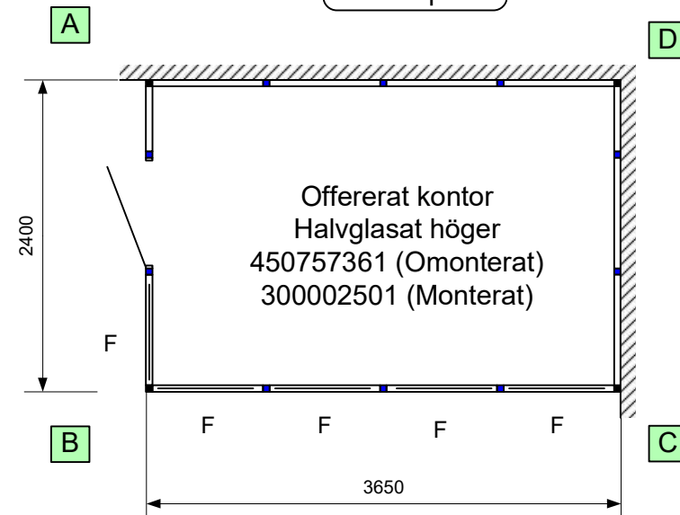
Bottenplan
