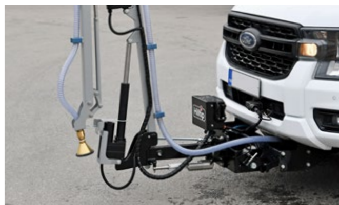
HWA-5 watering arm with Hilltip quick-hitch mounting system
