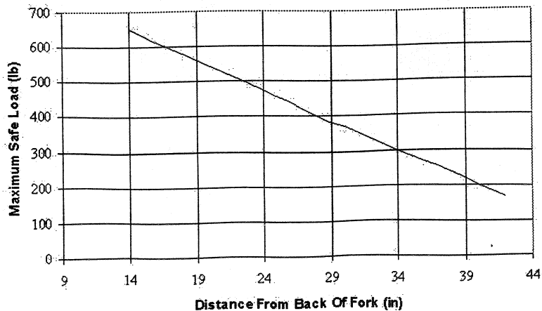
LOAD CAPACITY CHART 2100 Series Lift
